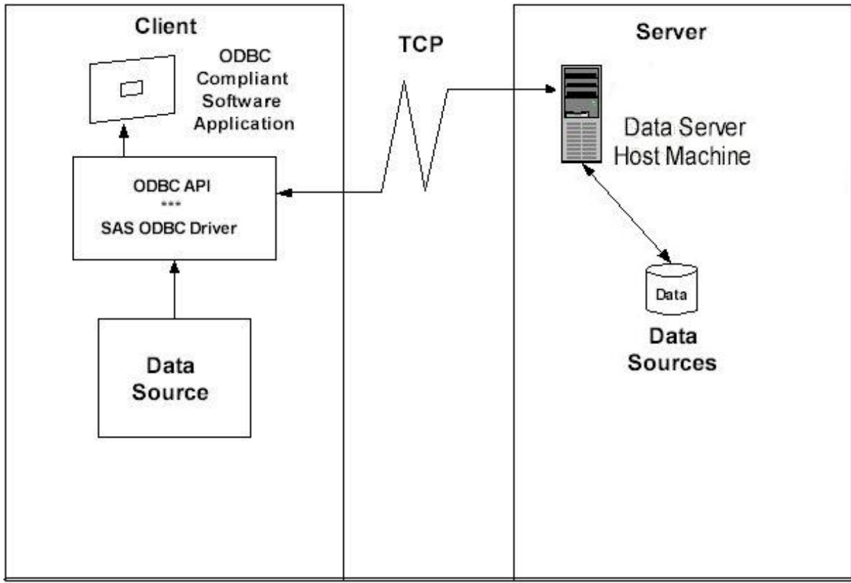
Configure ODBC to Connect SPD Server Client to SPD SNET Server
